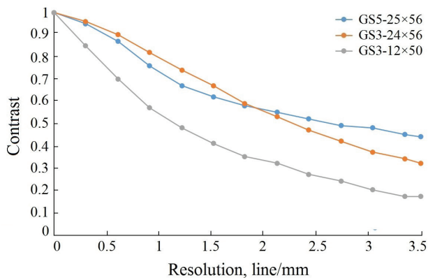
Figure 6 – Plot of the GS3-12x50, GS3-24x56, GS5-25x56 scopes at minimum magnification
