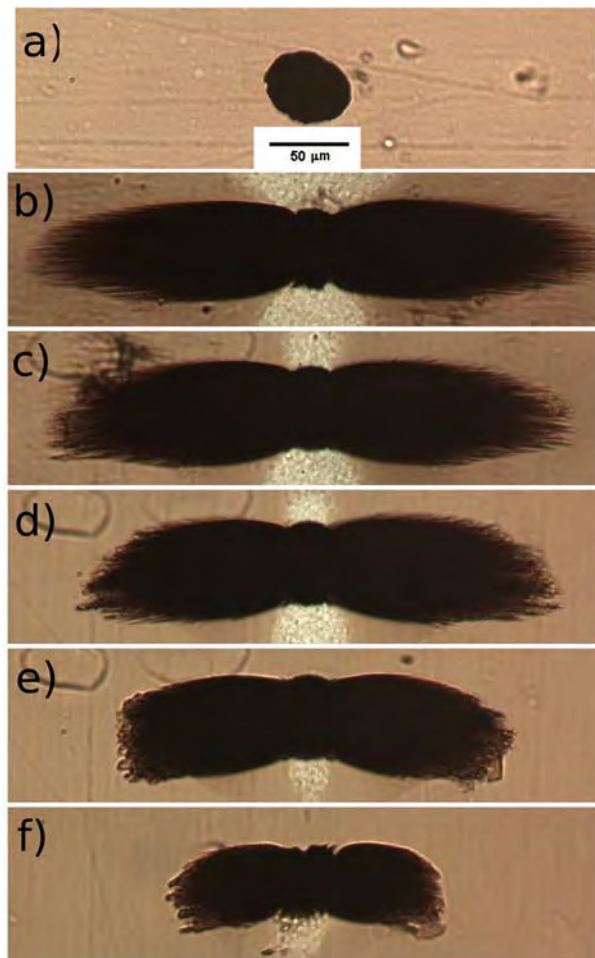
Fig.4. (Color online) Visualization of the nanocluster clouds in the transverse magnetic field H_0=12 kA/m at different flow speeds v_0 , equal to 1.67\cdot 10^{-4} m/s (b), 2.38\cdot 10^{-4} m/s (c), 5.95\cdot 10^{-4} m/s (d), 1.19\cdot 10^{-3} m/s (e) and 2.38\cdot 10^{-3} m/s. The snapshot (a) shows a bare nickel microparticle.
