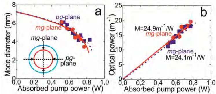
Fig. 2. Laser characteristics of Tm,Ho:KLuW in the hemispherical laser cavity (position: 13 cm away from the OC). (a) Mode diameter of the output beam vs. absorbed pump power, symbols: experimental data, curves: data fitting using the ABCD method, inset: scheme representing the distortion of the output laser beam profile (blue circle – near the threshold, red circle – at a high pump level). (b) Calculated optical power of the thermal lens (symbols) and the corresponding linear fits.
