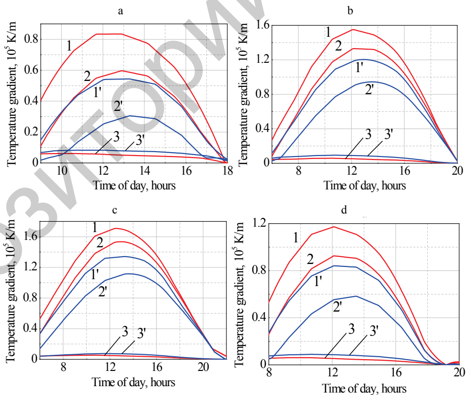
Fig. 7. The temperature gradients of CuInSe 2 solar cell at the upper (curves 1, 1') and lower (curves 2, 2') boundaries of the thermoelectric layer and at the upper (curves 3, 3') boundary of the photoelectric converter on the southeast side in the presence (curves 1, 2, 3) and the absence (curves 1', 2', 3') of the thermal insulation of the substrate ends in January (a), April (b), July (c) and October (d)
