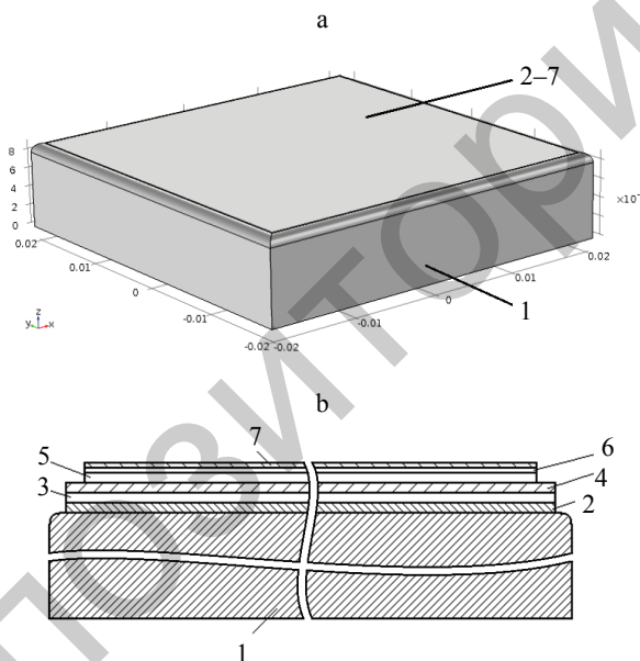
Fig. 1. The thin-film solar cell structure (a) and its cross-section (b): 1 – substrate; 2 – first electrode layer; 3 – thermoelectric layer based on \text{CuInSe}_2 ; 4 – second electrode layer; 5, 6 – photoelectric converter consisting of \text{CuInSe}_2 and CdS layers respectively; 7 – transparent electrode
