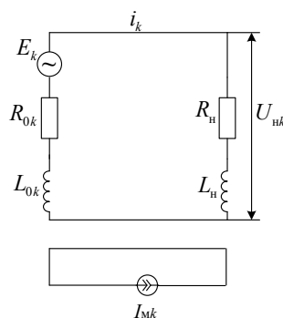
Fig. 2. The equivalent circuit diagram for the k^{\text{th}} working contour of the reciprocating electric generator operating for active-inductive loading: L_{0k}, R_{0k} – inductance and active resistance of the working winding; E_k – EMF of motion; I_{mk} – ideal current source
