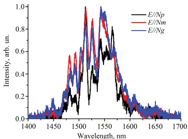
Figure 7 – Polarised luminescence spectrum of the Er,Yb:YMB0 crystal
