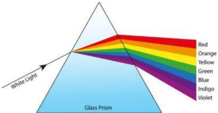
Figure1: Separation of White Light into a Spectrum
