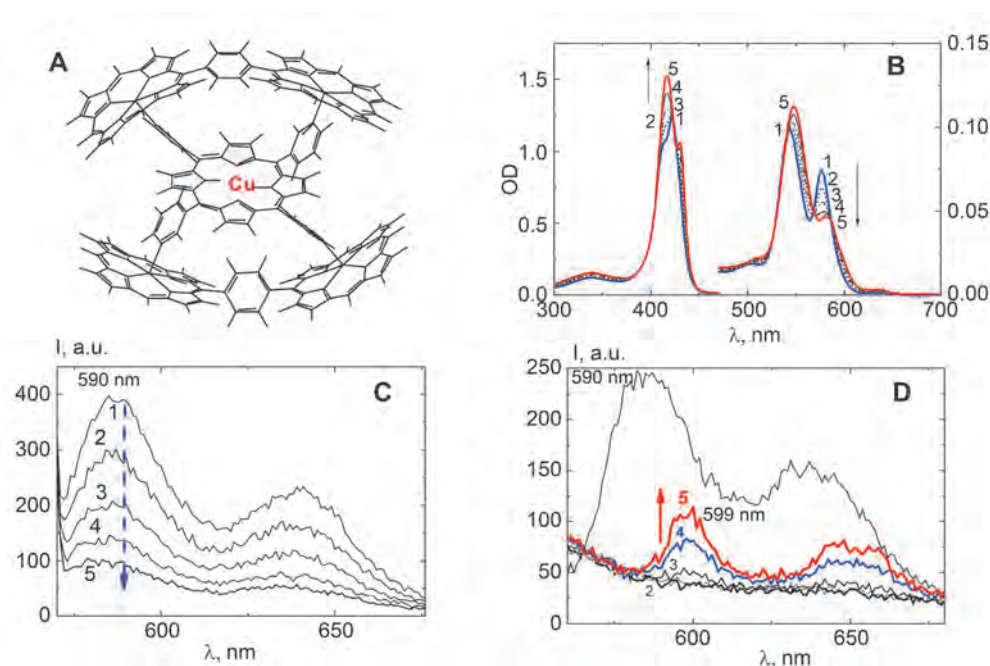
Figure 4. Formation and spectral properties of pentad 2(ZnOEP) 2 Ph@CuP(mPyr) 4 in toluene. A: Mutual arrangement of the dimer (ZnOEP) 2 Ph and extra-ligand CuP(mPyr) 4 . For clarity, \beta -ethyl substituents in (ZnOEP) 2 Ph are omitted. (HyperChem software, release 4.0 geometry optimization with semiempirical PM3 method). The symbol \otimes is used in order to show what interacting subunits (dimer and extra-ligands) are bound together.
