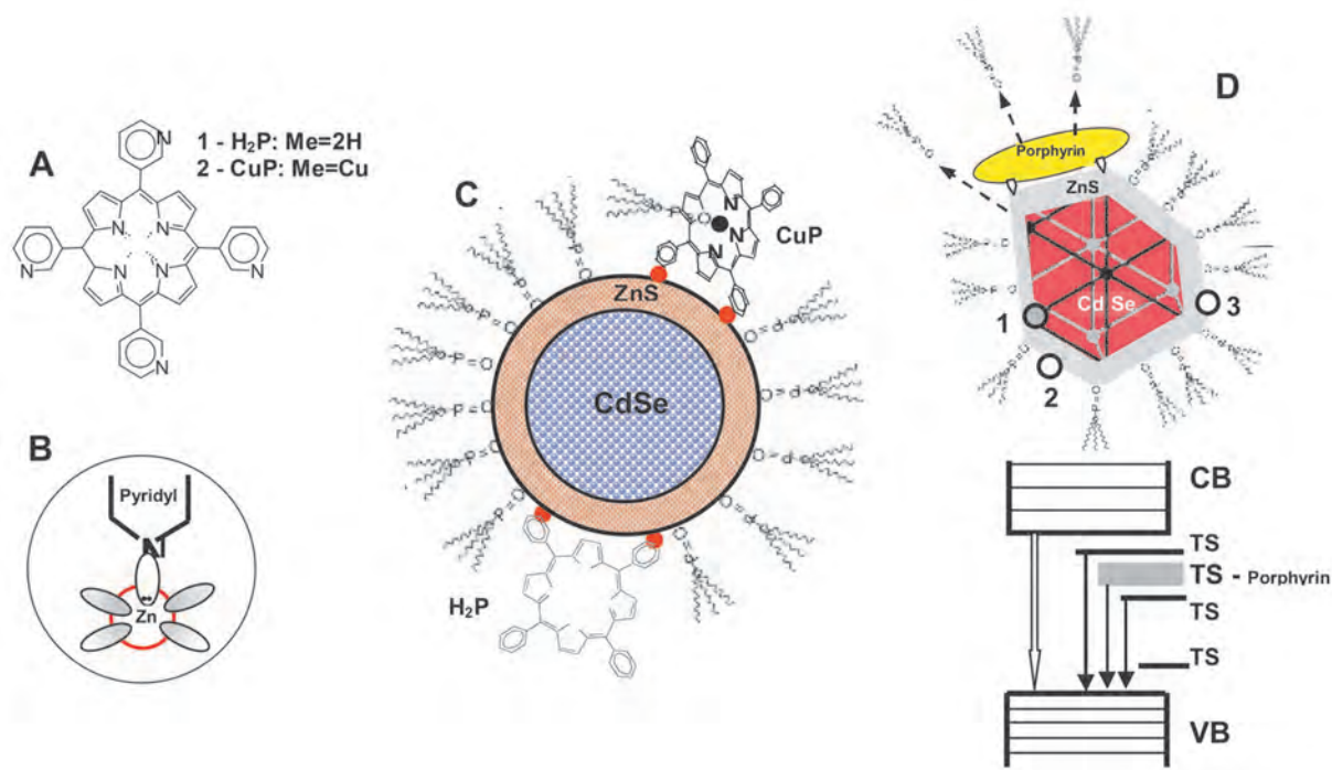
Figure 9. A: Chemical structures of 5,10,15,20- meso-meta -pyridyl porphyrins [free base H 2 P (1) and CuP (2)]. B: Coordination scheme of porphyrins attachment to the ZnS shell via pyridyl N...Zn interaction. C: mutual arrangement of H 2 P and CuP molecules with respect to the QD surface. Nitrogen lone pair orbitals (participating in Zn-N coordination) are indicated by a red dot. Capping ligands, trioctylphosphine oxide molecules (TOPO) are depicted also. Additional extra-ligation of TOPO molecule to the central Cu atom of CuP molecule is shown also (see explanation in the text). D: Schematic presentation of “QD-Porphyrin” nanoassembly as well as arbitrary excitonic and trap states (TS) and main relaxation pathways. An induced ligand (TOPO) detachment is shown by dashed arrows. 1 is a hole trap, 2 and 3 are electron traps. Partly adopted from refs. [99,123]
