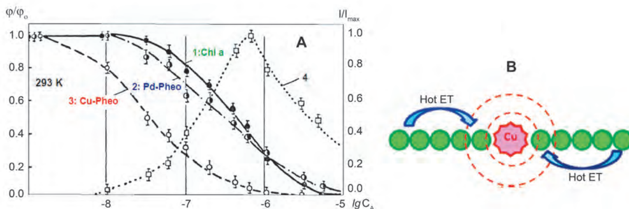
Figure 8. A: Dependence of the relative quantum efficiency ( \phi/\phi_0 ) of fluorescence for protochlorophyll a aggregate ( \lambda_{exc}=460 nm, \lambda_{det}=630 nm) upon mixed association with chlorophyll a (1), Pd-pheophytin a (2) and Cu-pheophytin a (3) being observed at the increase of the molar concentration of Chl a , Pd-Pheo and Cu-Pheo ( C_A ) to the initial solution of protochlorophyll ( C_0=1 \times 10^{-5} M). 4 – relative intensity ( I/I_{max} ) of chlorophyll a fluorescence ( \lambda_{exc}=693 nm, \lambda_{det}=693 nm) in mixed aggregates with protochlorophyll a . B: Scheme of d- \pi exchange distant effects in mixed aggregates caused by Cu ion of Cu-pheophytin a and enhanced by “hot” energy transfer among aggregated host protochlorophyll a molecules.
