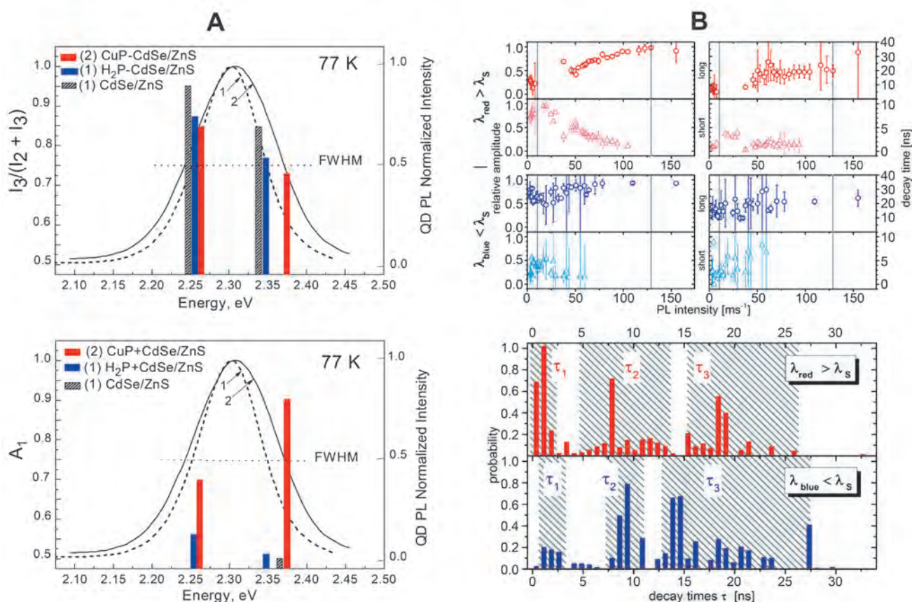
Figure 11. QD photoluminescence analysis for ensemble experiments (A) single quantum dots (B) based on experimental results presented in [99] . A: Relative PL intensities I_3 / (I_2 + I_3) (top) and normalized amplitudes A_1 (bottom) for solutions of pure CdSe/ZnS QDs and QDs in "QD-CuP" or "QD- \text{H}_2\text{P} " nanoassemblies at 77 K. Normalized QD PL bands are shown as broken lines for pure CdSe/ZnS (1) or QDs in \text{H}_2\text{P-CdSe/ZnS} (1) and as full lines for \text{CuP-CdSe/ZnS} (2) nanoassemblies at 77 K. FWHM is the full width of half-maximum of the corresponding bands. B: Variations of PL decay times (two-exponential fits) during a blinking time trace for single CdSe/ZnS QDs on a quartz substrate at room temperature upon detection in the red and blue range of the PL band, respectively. Data are presented for amplitudes and lifetimes detected for the PL of one single QD in 2 different spectral detection channels (top) and for 20 single QDs depending on the spectral detection channel (bottom). "Grouping" of decay times into 3 typical time regimes \tau_i is indicated by shaded areas.
