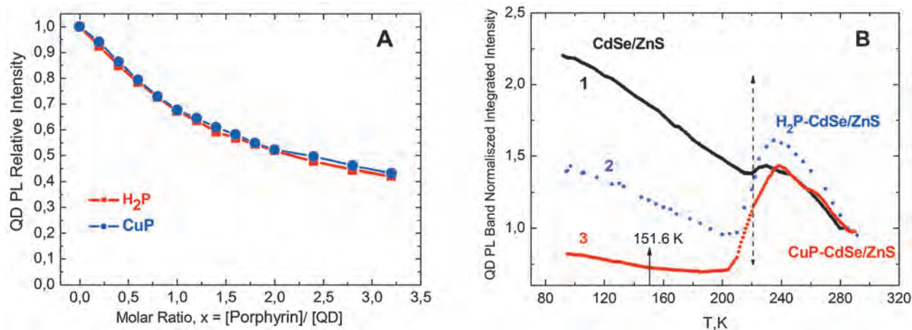
Figure 10. A: Photoluminescence quenching for TOPO-capped CdSe/ZnS QDs upon titration by \text{H}_2\text{P} and \text{CuP} molecules in toluene at 295 K) for various attached porphyrin molecules. d_{\text{CdSe}} = 2.6 nm, 2 monolayers ZnS, \lambda_{\text{exc}} = 440 nm, \lambda_{\text{reg}} = 554 nm. B: Temperature dependence of normalized QD PL intensity ratio, for TOPO-capped CdSe/ZnS (1) as well as for QDs in \text{H}_2\text{P-CdSe/ZnS} (2) and \text{CuP-CdSe/ZnS} (3) nanoassemblies at molar ratio x=1 in a methylcyclohexane-toluene (6:1) mixture for \lambda_{\text{exc}} = 450 nm. Temperature T_{\text{crit}} \approx 220 K (phase transition assigned to the capping TOPO layer) are indicated by dashed arrow. The temperature of the glass transition for the methylcyclohexane/toluene (6:1) mixture at 151.6 K is shown by an arrow (full line). Partly adopted from refs. [94,99,123]
